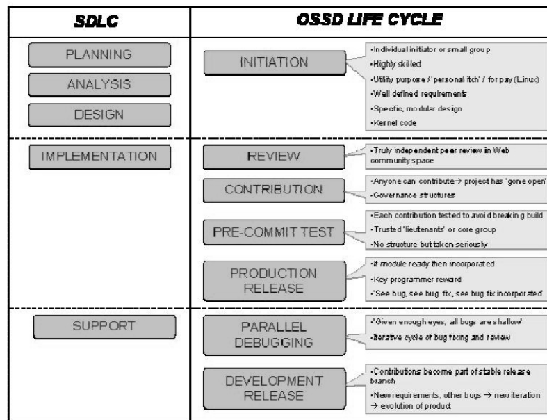
Figure 5: Model of Rinette Roets et al [09] and its comparison with SDLC
