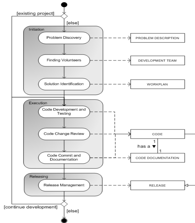
Figure 2. OSS Development Process (source wikipedia)
